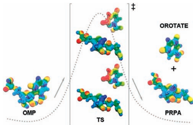
Figure 7. Reaction coordinate for the conversion from OMP to the products orotate and 5-phosphoribosyl 1-phosphonoacetic acid (PRPA). The transition state structures of Pf OPRT and Hs OPRT are shown. MEP surfaces were generated by the CUBE subprogram of Gaussian 98 and visualized using Molekel 4.0 at a density of 0.2 electron/Å 3 .
