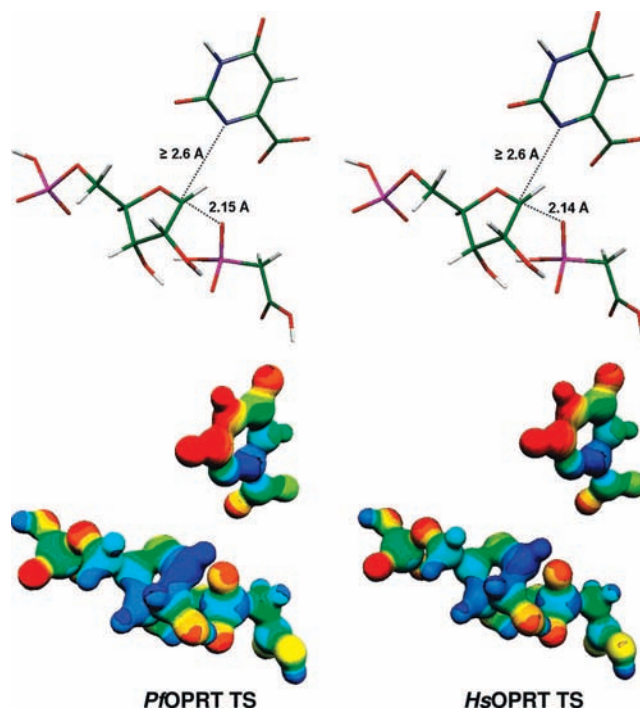
Figure 6. Transition state structures of Pf OPRT and Hs OPRT (stick and MEP modes). The transition state structures were determined in vacuo by hybrid density functional theory implemented in Gaussian 98 using B3LYP functional and the 6-31G(d,p) basis sets. The distances in the reaction coordinate (C1'-N1 and C1'-O PA ) for Pf OPRT and Hs OPRT transition states are shown. The molecular electrostatic potential (MEP) surfaces were generated by the CUBE subprogram of Gaussian 98 and are visualized using Molekel 4.0 at a density of 0.2 electron/Å 3 . Blue is electron deficient (cationic) and red is electron rich (anionic) in this rendering and in Figure 7.
