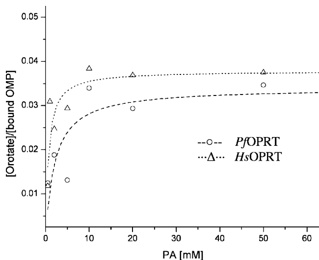
Figure 4. Forward commitments to catalysis by PfOPRT and HsOPRT . Isotope trapping experiments were performed to measure the forward commitment factors. [1, 3- 15 N 2 , 5'- 14 C]OMP was preincubated with OPRTs for 10 s and then rapidly mixed with chase buffers including cold OMP and various concentrations of PA. After five catalytic turnovers, the generated products were isolated by charcoal column chromatography and analyzed on the basis of the total radioactivity. The fractions of product formed versus bound substrate at time zero were plotted against PA concentrations. Forward commitment factors were calculated on the basis of C_f = (Y_{\max})/(1 - Y_{\max}) to give the C_f of PfOPRT (-○-) of 0.035 \pm 0.006 and C_f of HsOPRT (•••Δ•••) of 0.042 \pm 0.003 (see Experimental Methods for details).
