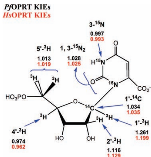
Figure 5. Intrinsic KIEs for Pf OPRT and Hs OPRT. The positions for isotopic labeling are indicated in the substrate OMP.
