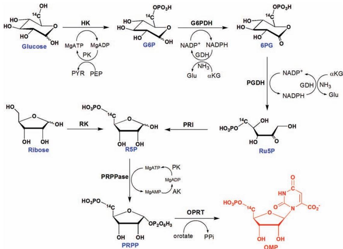
Figure 3. Synthesis of isotopically labeled OMPs using [5'- 14 C]OMP as an example. [1'- 14 C]-, [1'- 3 H]-, [2'- 3 H]-, [4'- 3 H]-, [5'- 14 C]-, [5'- 3 H 2 ]-, [1, 3- 15 N 2 , 5'- 14 C]-, [3- 15 N, 5'- 14 C]-, and [1, 3- 15 N 2 , 1'- 14 C]OMP were prepared from isotopically labeled riboses, glucoses, and orotates through one-pot, stepwise enzymatic reactions. The enzyme mixtures used for the synthesis contain ribokinase (RK), hexokinase (HK), glucose-6-phosphate dehydrogenase (G6PDH), phosphogluconic acid dehydrogenase (PGDH), L-glutamic dehydrogenase (GDH), phosphoriboisomerase (PRI), adenylate kinase (AK), pyruvate kinase (PK), phospho-D-ribosyl-1-pyrophosphate synthase (PRPPase), and orotate phosphoribosyltransferase (OPRT).
